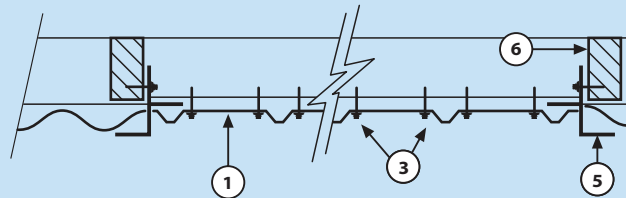
Framed Side Light Horizontal Section Figure 32
