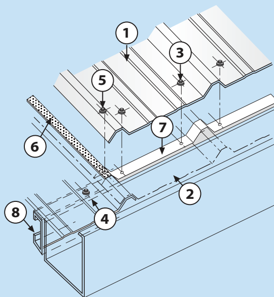
Bottom Edge SunSky Installation with Profiled Closure Strip Figure 22
