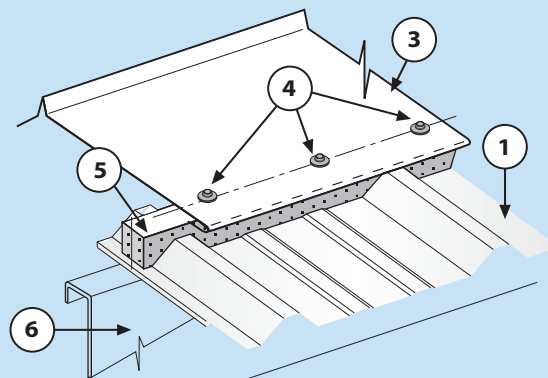
Sheet-Metal Ridge Cap Fastening Figure 24a
