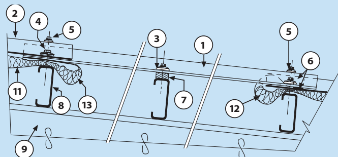
Length Section Detail
